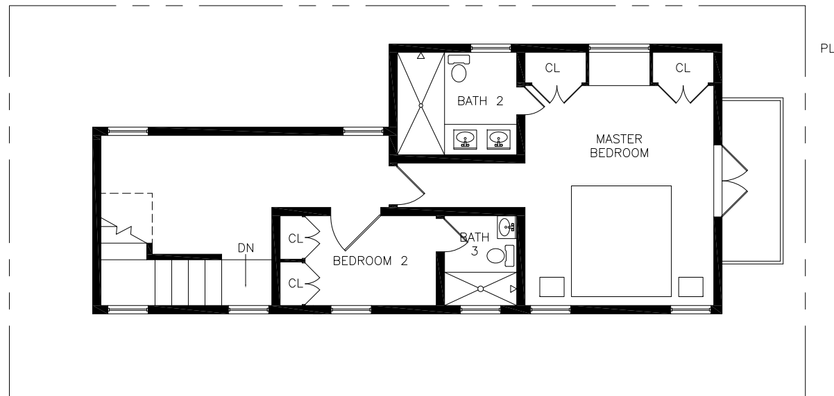
2 SECOND FLOOR 528# SCALE: 1/8"=1'-0"
