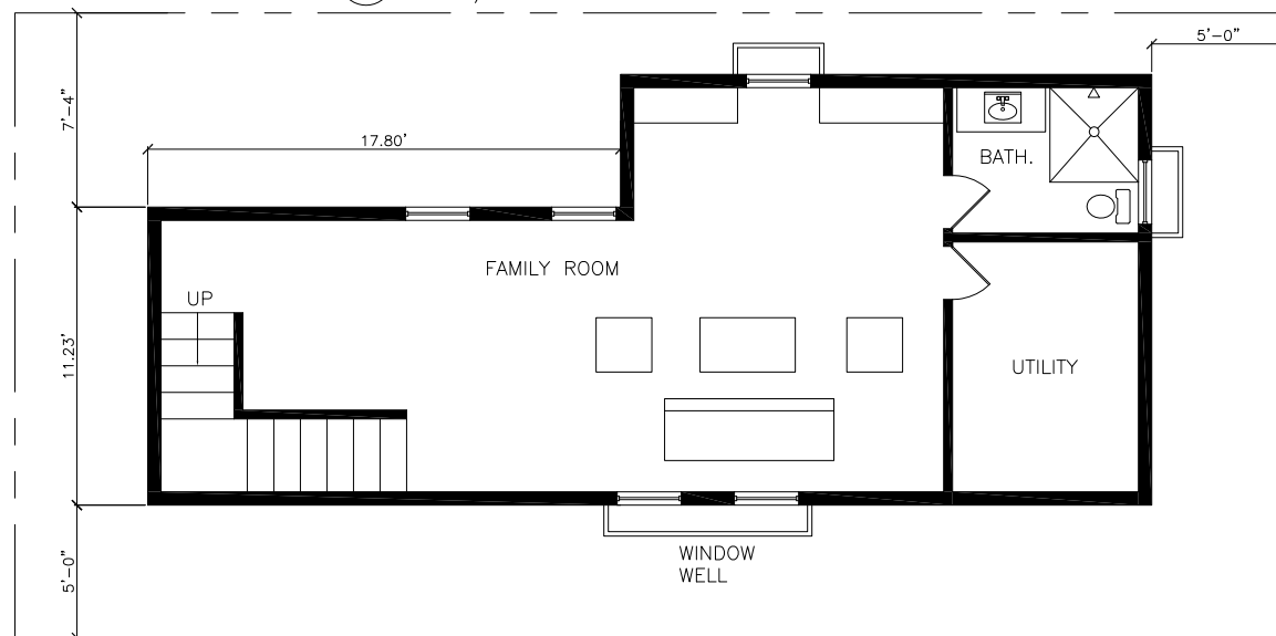
1 BASEMENT SCHEME 2 528# SCALE: 1/8"=1'-0"
