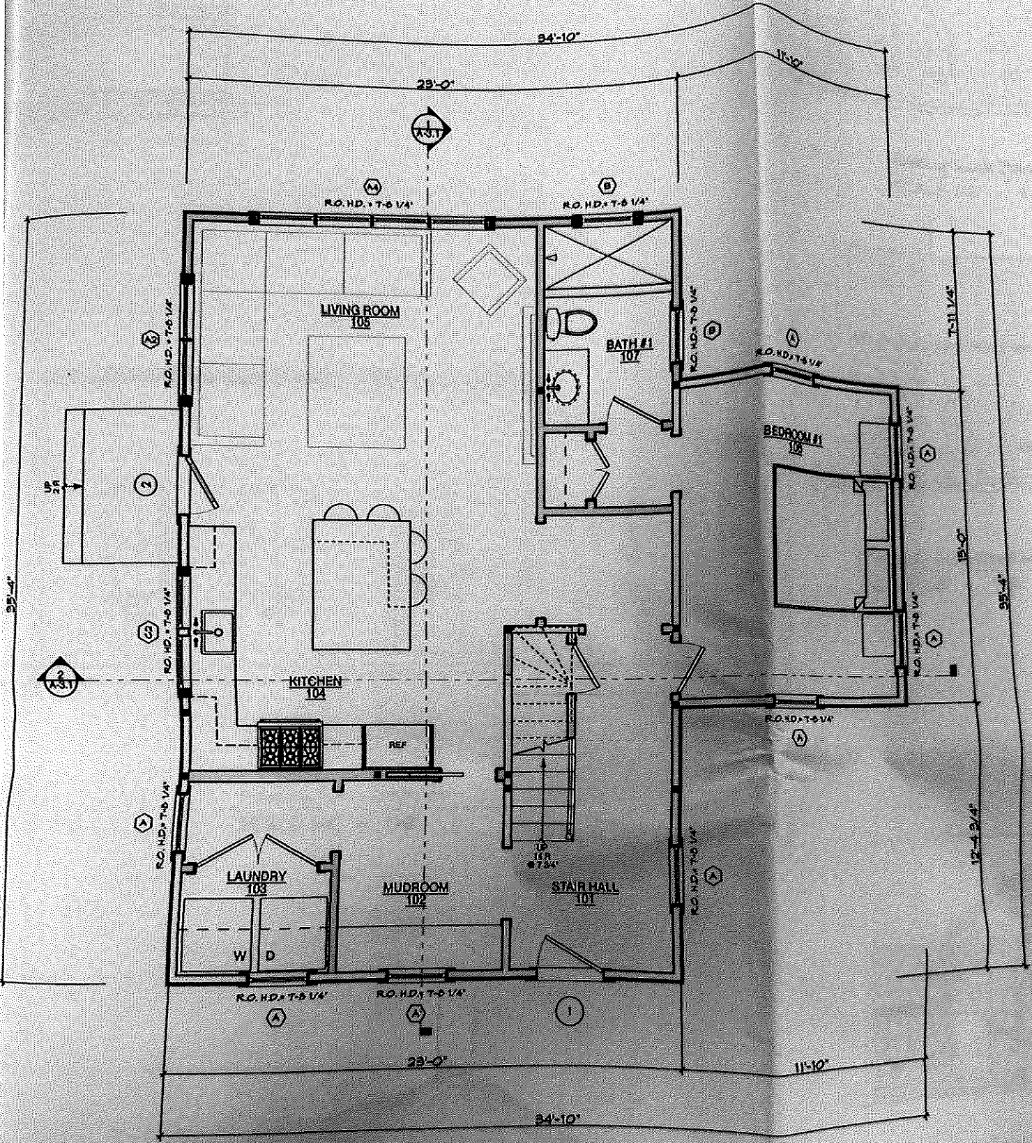
1 First Floor Plan SCALE: 1/4" = 1'-0"
